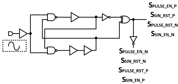
Figure 6 Four-phase source: a) Circuit diagram implemented in a parallel buffer chain; b) Simulation result.
