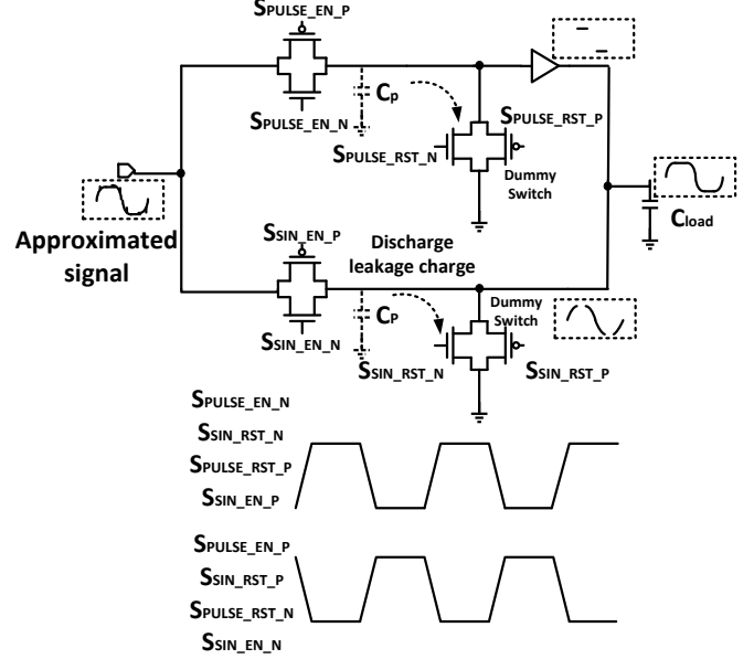
Figure 5 The circuit diagram of clock MUX.
